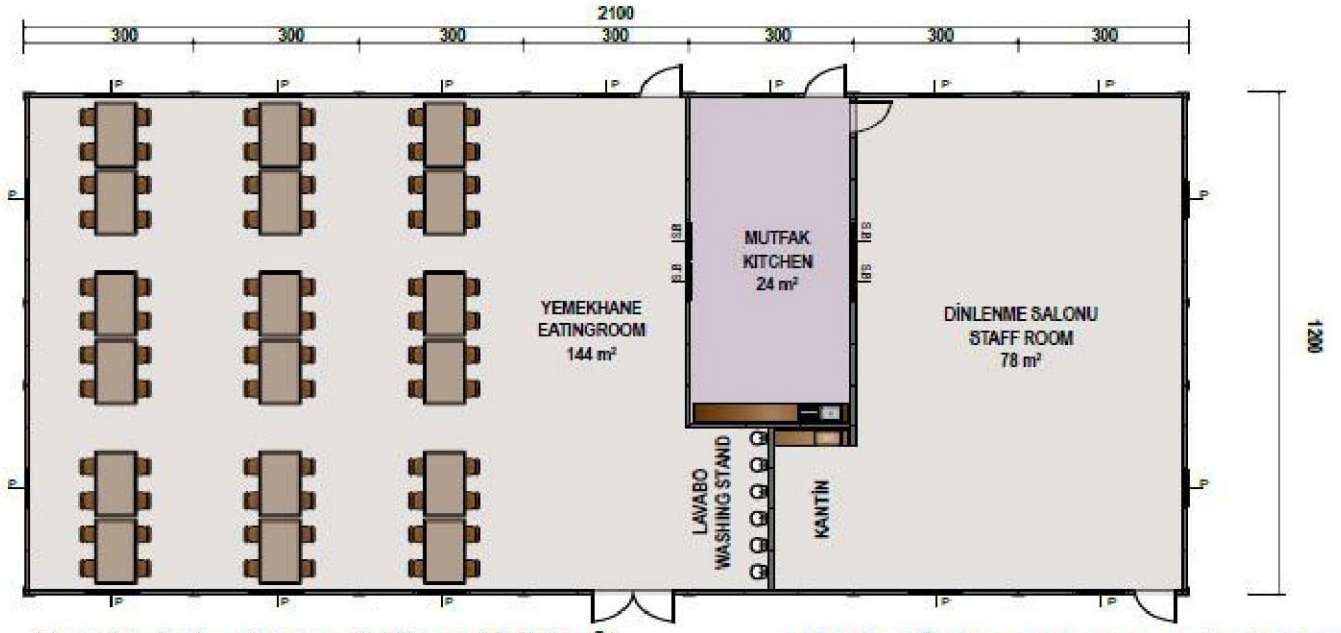
Zemin kat - Ground Floor (252m 2 )
